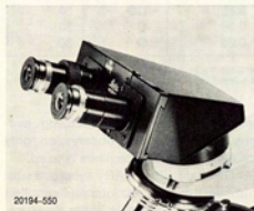
Fig. 5 Inclined binocular pol tube S 20 For orthoscopic observation. Conoscopy possible only with the pinhole stop, which is inserted in the eyepiece tube instead of the eyepiece.
