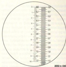
Fig. 17 Division of the graticule in the eyepiece and image of the stage micrometer
