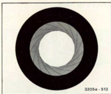
Fig. 8 Image of the aperture diaphragm It is visible in the tube after removal of the eyepiece.
