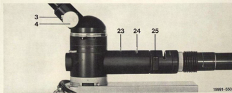
Fig. 24 Incident-light device for the SM-LUX-POL 3 Pinhole stop, 4 Bertrand lens, 23 Field diaphragm, 24 Aperture diaphragm, 25 Polarizer Analyser not visible in Fig. 24, see Fig. 1.
