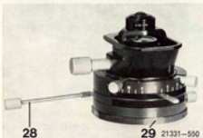
Fig. 8a Condenser 702 fi 28 Adjustment key 29 Index lines
