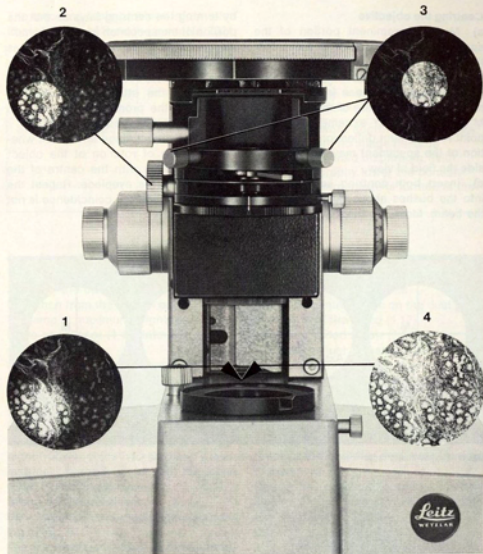
Fig. 9 Centring the field diaphragm
